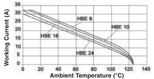
HBE CRIMP TERMINATED: 2.5 mm 2 (14 AWG)
